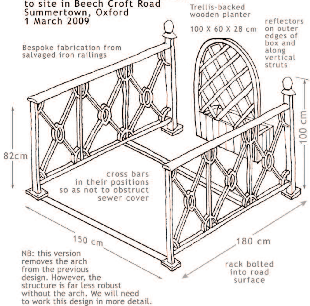
ITEMS 12, 14 : Triple-hoop or 'Sheffield' cycle rack
